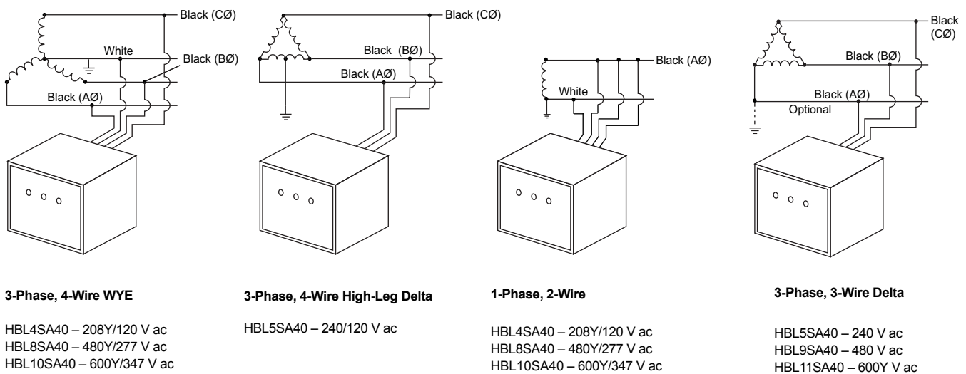
Figure 2: Wiring
