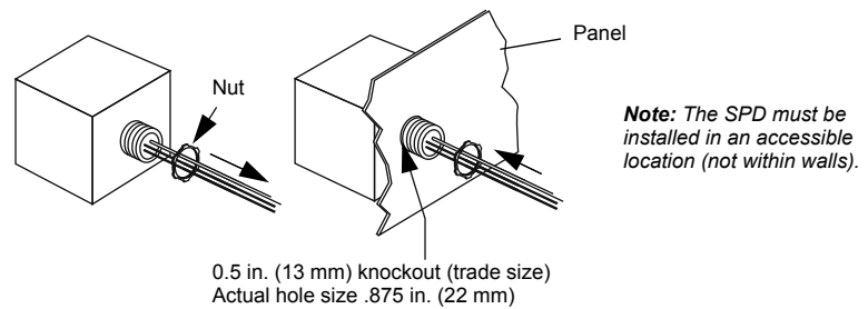
Figure 1: Mounting
